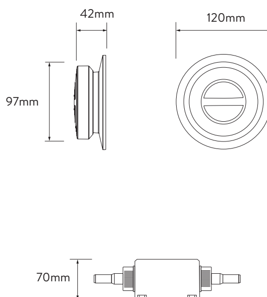
CONTROLLER
